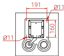
MOUNTING HOLES SPACING
